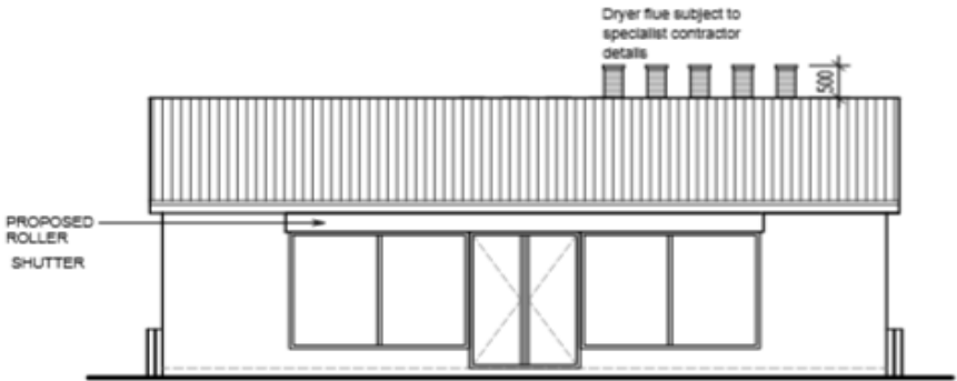
PROPOSED FRONT ELEVATION - A
