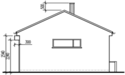
PROPOSED SIDE ELEVATION - B
