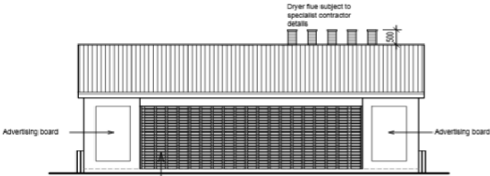
PROPOSED FRONT ELEVATION - A
